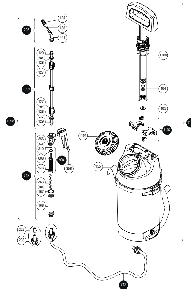
LOW-VOLUME WEED-KILLERS ELBOW Reference 8.34.60.935
